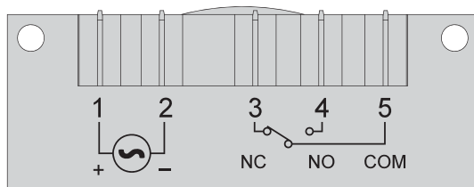
WIRING TERMINALS (polarity marked on DC models)
